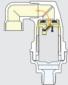
Dissolved air is accumulated in the valve, when released the float drops down
